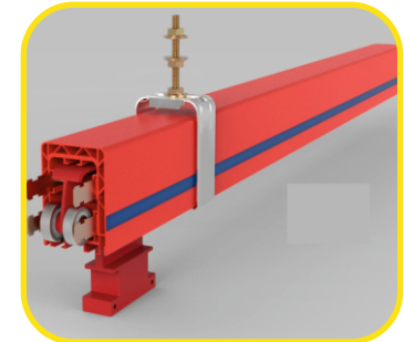
CLOSED BUSBAR
